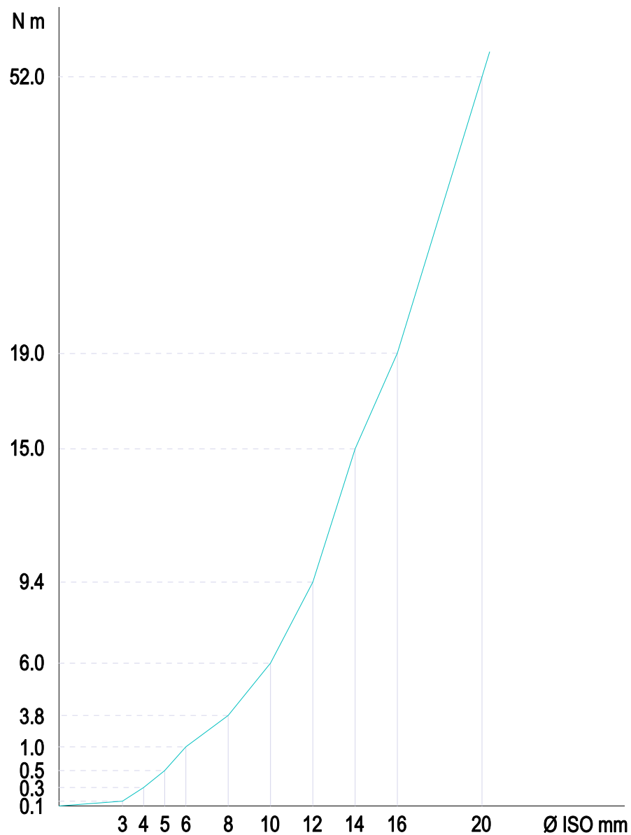
*Tightening torque at break (Nylon 66)
